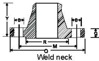
Weld neck
